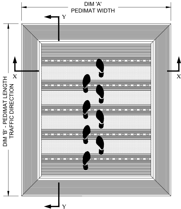
TYPICAL PLAN VIEW
