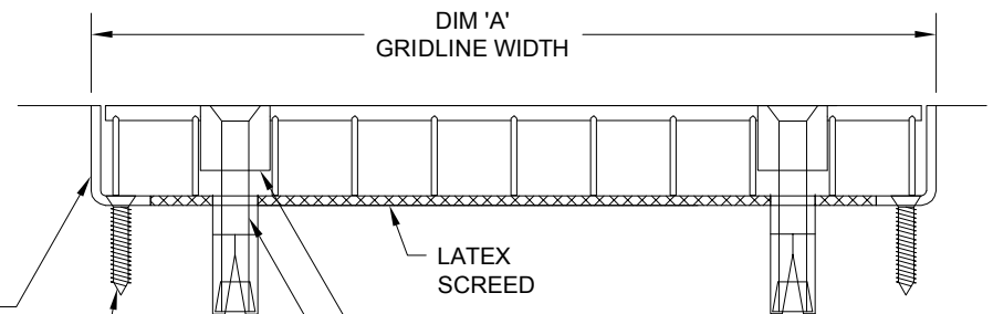
SECTION Y-Y
