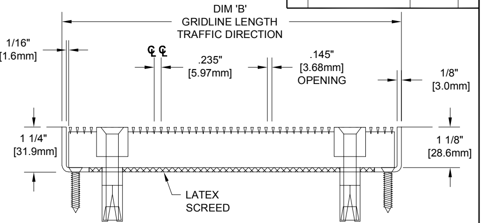
SECTION Y-Y
